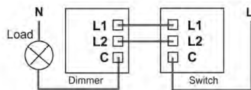
Figure 3. Using a 2-Way Dimmerswitch (For single switches or each module of a multi-gang)
